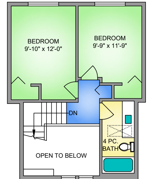
UPPER FLOOR 444 SQ. FT. 8'-0" CEILING HEIGHT
