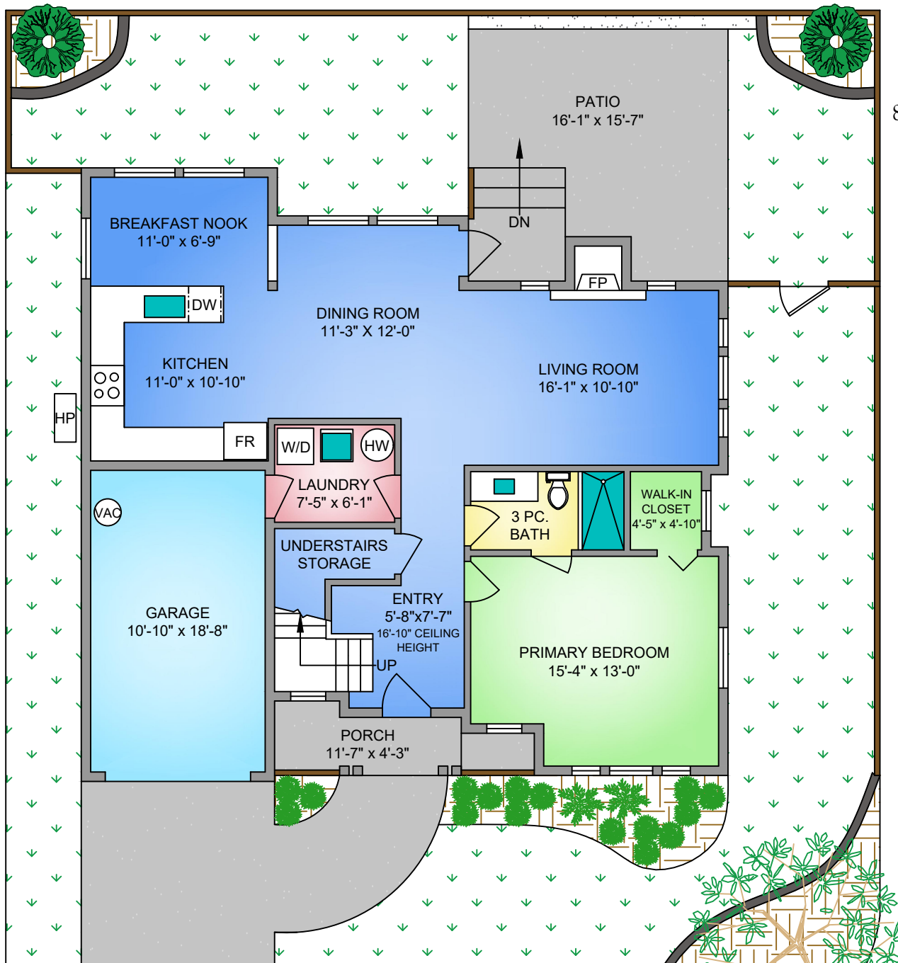
MAIN FLOOR 1073 SQ. FT. 8'-0" CEILING HEIGHT
