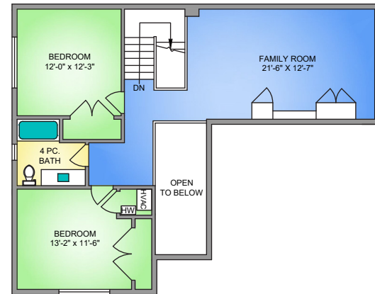
UPPER FLOOR 901 SQ. FT. 8'-0" CEILING HEIGHT
