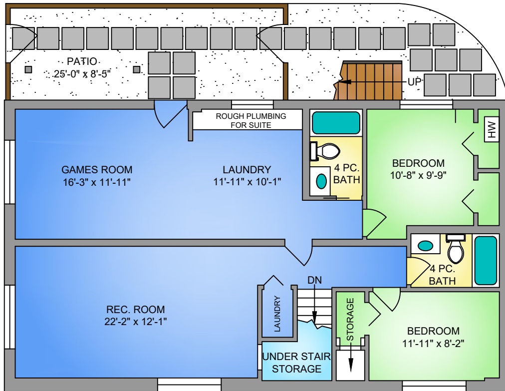
LOWER FLOOR 1230 SQ. FT. 8' CEILING HEIGHT
